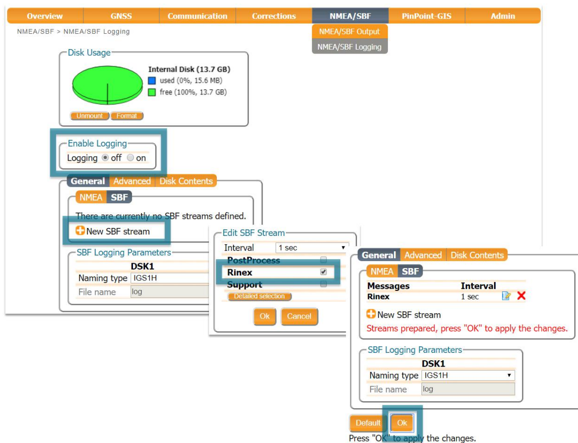
Figure 6-1: logging the SBF blocks necessary for RINEX conversion
