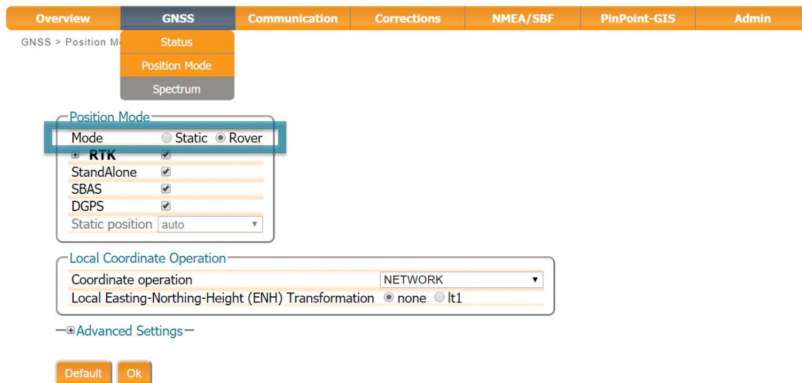
Figure 4-1: By default, the Altus NR3 is configured as a rover with all positioning modes enabled
