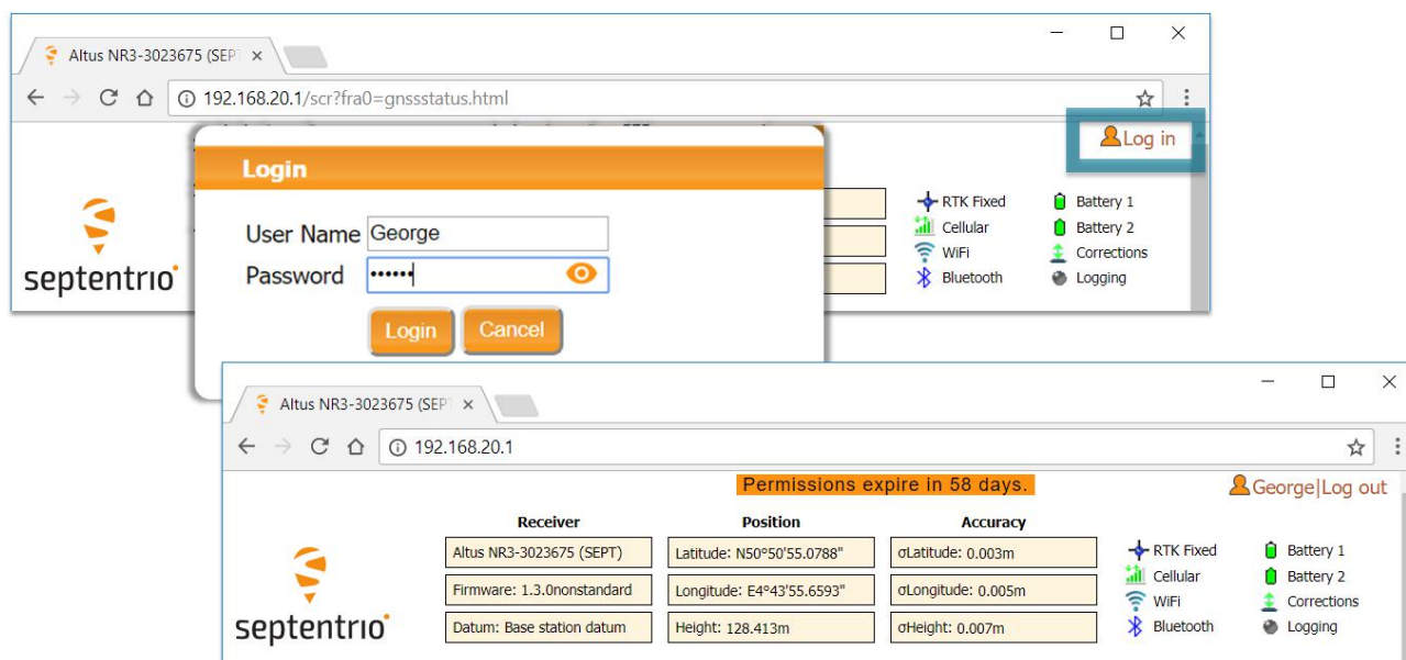
Figure 6-15: Logging in to the Altus NR3 web interface
