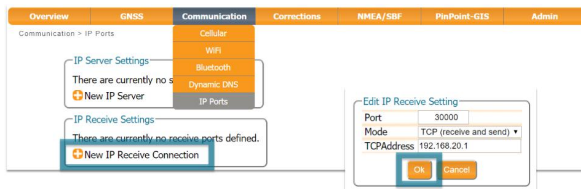
Figure 4-16: Configure the rover receiver to listen for the diff corr output from the Base station
