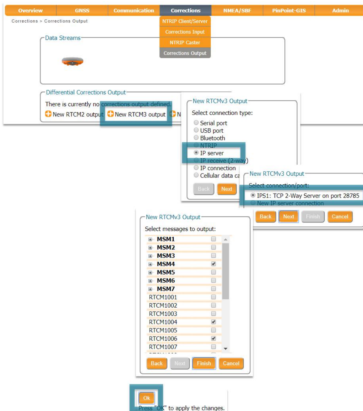
Figure 5-9: Output RTCMv3 diff corr on the configured TCP/IP server port of the Base station receiver
