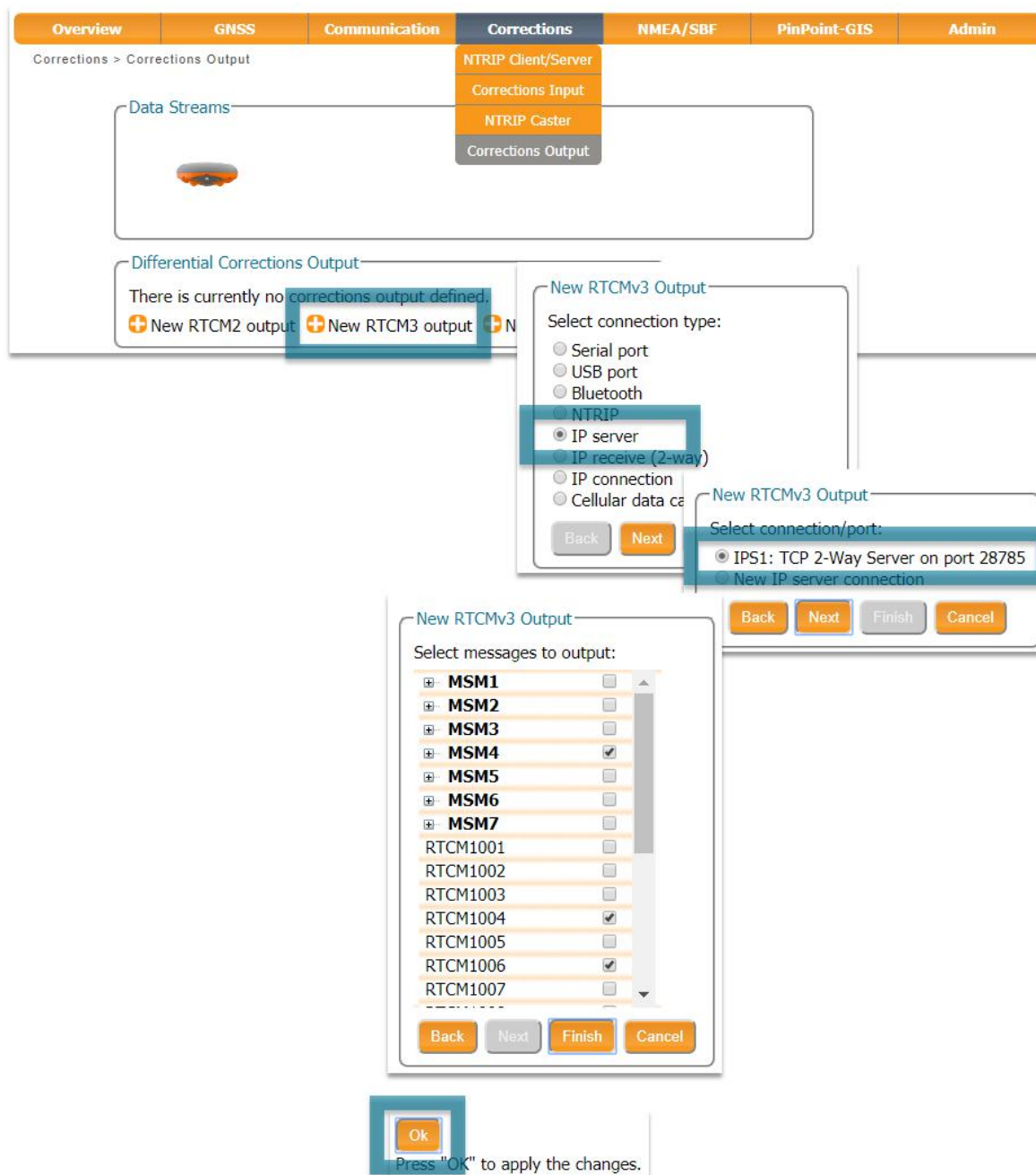
Figure 5-14: Output RTCMv3 diff corr on the configured TCP/IP server port of the base station receiver
