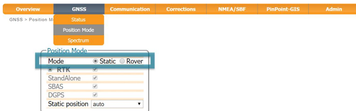
Figure 5-1: Setting the Altus NR3 base station position to static
