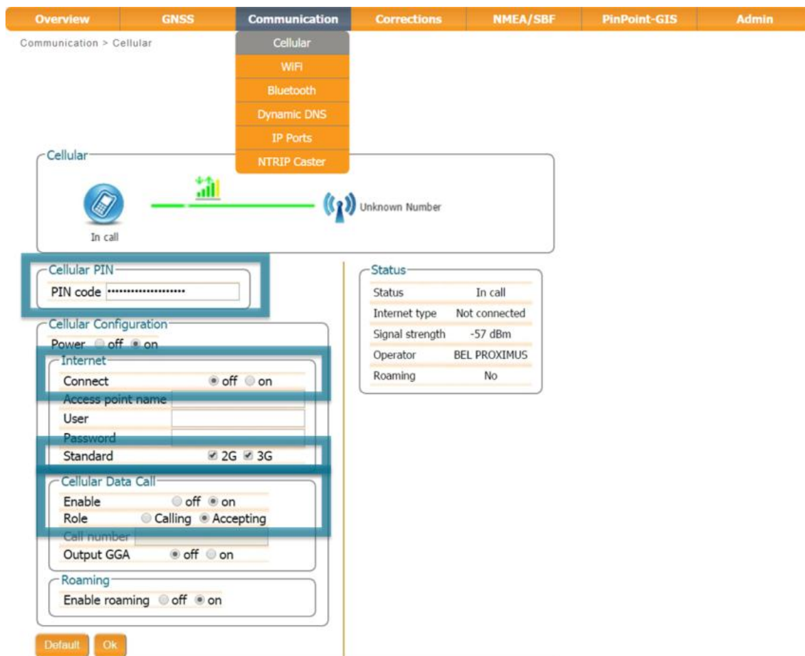
Figure 4-7: Configuring the Base station receiver to receive a data call from the rover receiver
