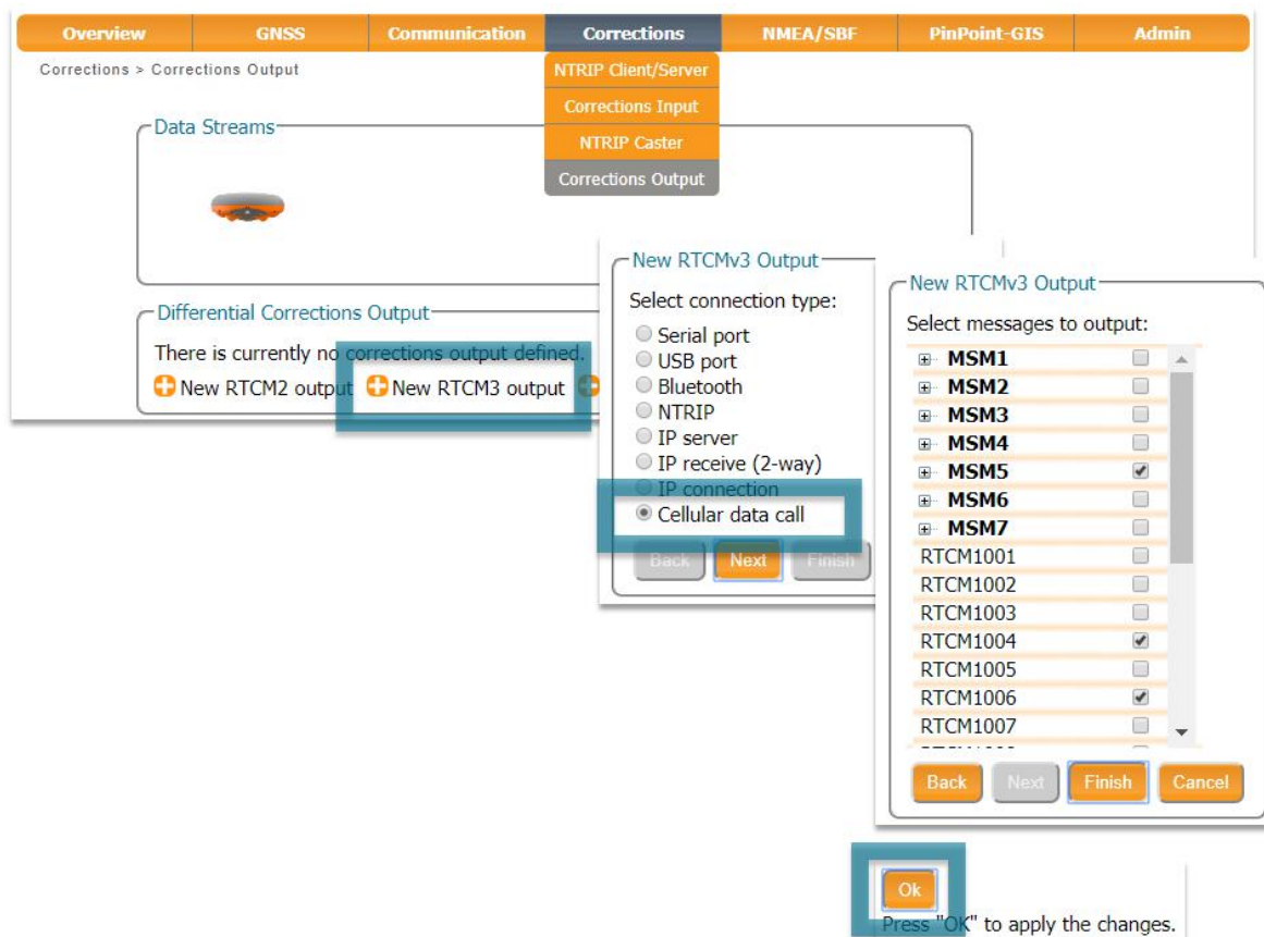
Figure 5-5: Output of RTCMv3 differential corrections over the DC1 connection of the base station receiver
