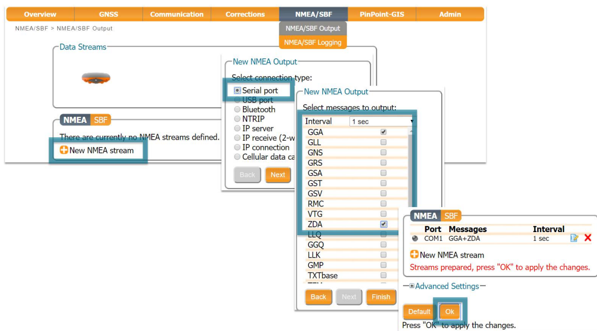
Figure 4-19: example showing output of NMEA GGA and ZDA over the serial COM connection
