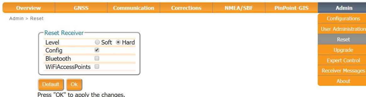
Figure 6-10: Admin - Reset
